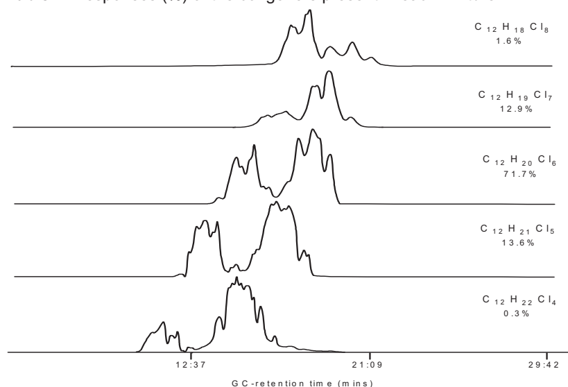
Figure 1. Elution profiles of the C 12 -chlorinated alkanes, determined by monitoring their respective [M–Cl] – ion. The relative abundance of each formula group is also shown.
